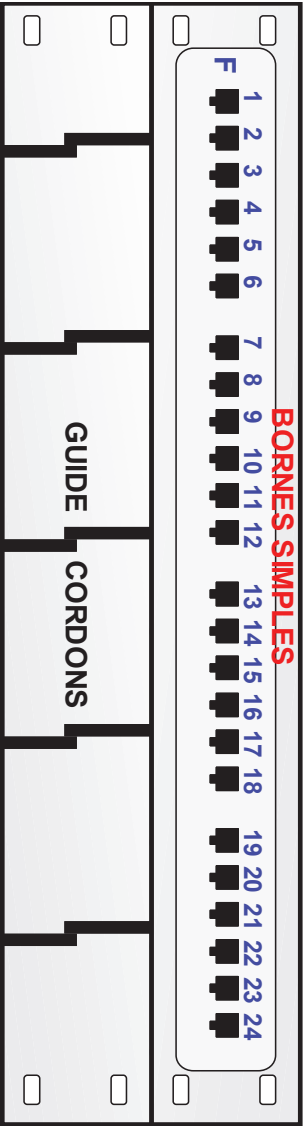
BLOC : ORGANISATION / NUMEROTATION 1u = 24 RJ, 1u = 1 guide cordons
