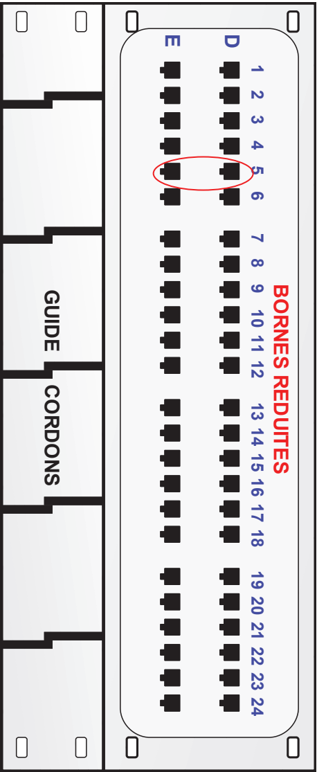
BLOC : ORGANISATION / NUMEROTATION 2u = 48 RJ, 1u = 1 guide cordons
